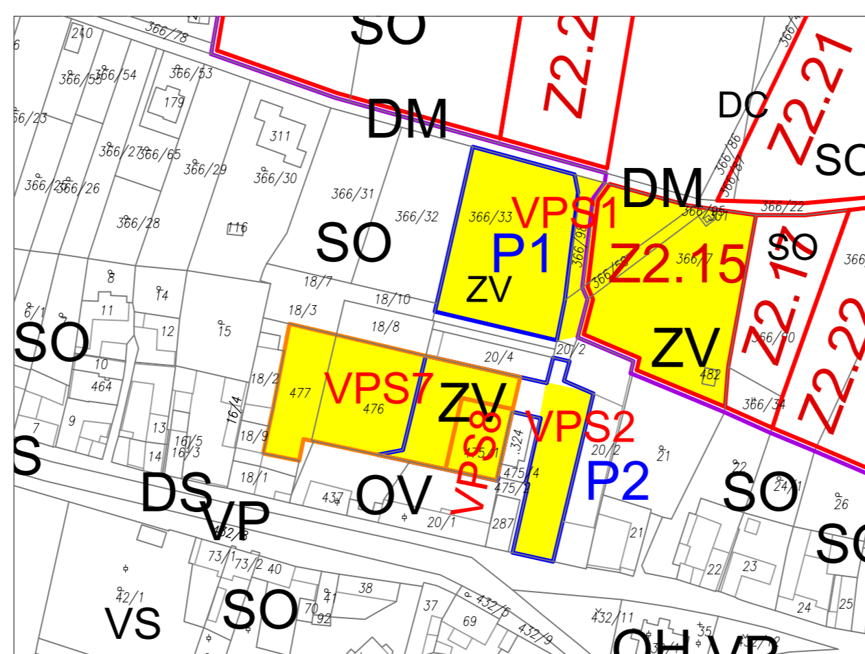
DETAIL M 1:2000
